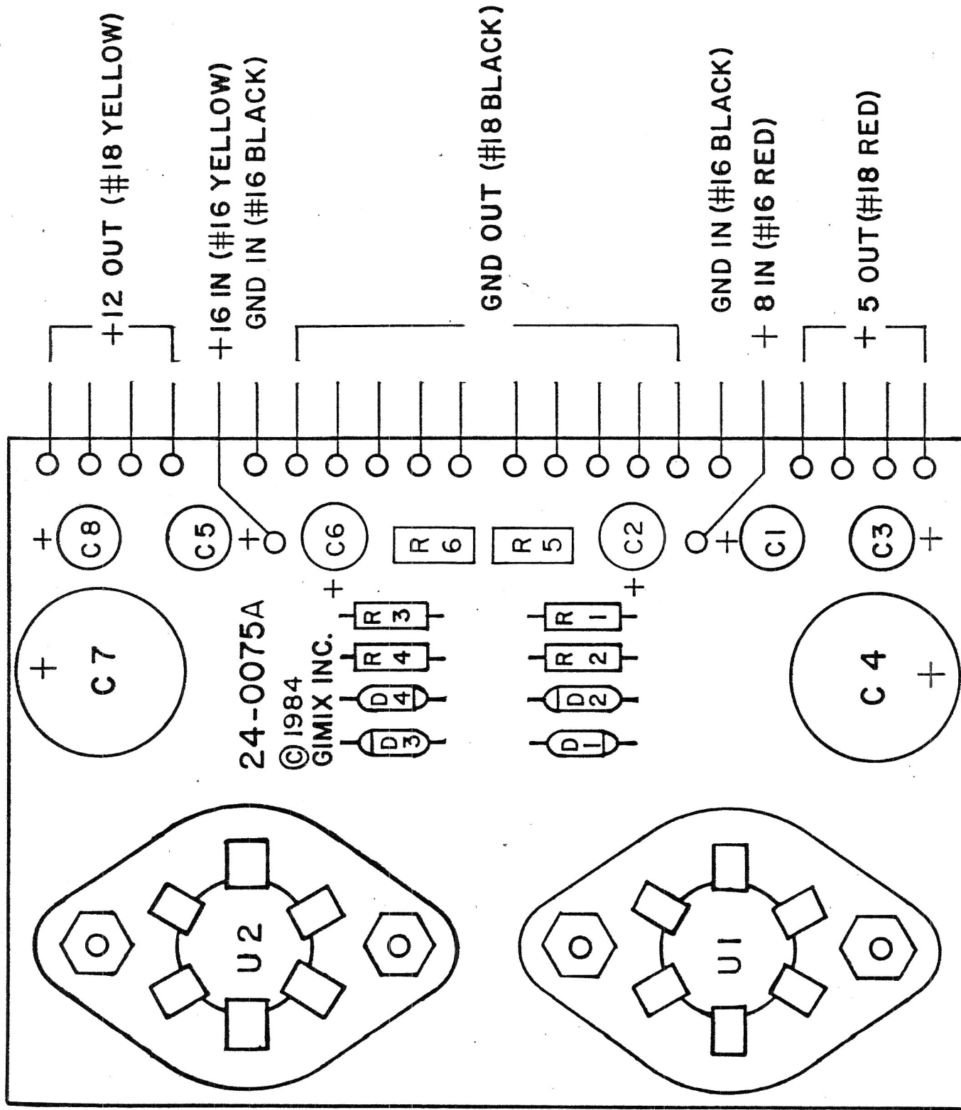
COMPONENT LAYOUT
